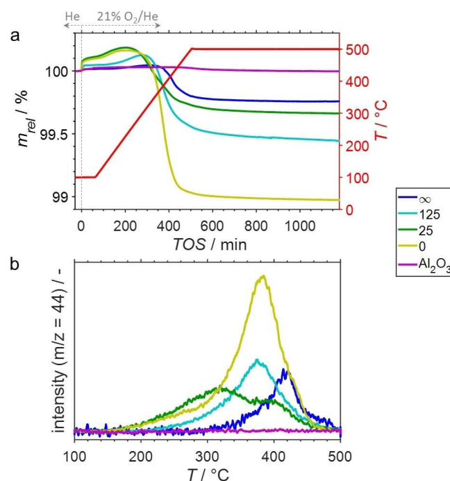
Figure 1. (a) Sample weight relative to the weight prior to exposure to 21 % \text{O}_2 /He at 100 °C and (b) formation of \text{CO}_2 during temperature programmed oxidation ( 1^\circ\text{C min}^{-1} ) of spent SCALMS with atomic Ga/Rh ratios of 25 and 125, the spent Ga/ \text{Al}_2\text{O}_3 (Ga/Rh = \infty ) and Rh/ \text{Al}_2\text{O}_3 (Ga/Rh = 0) reference catalysts, as well as the bare \text{Al}_2\text{O}_3 support material as monitored via high-resolution thermogravimetry coupled with mass spectrometry. All catalysts were previously applied in propane dehydrogenation at 450 °C. Conditions of the experiment: He flow 100\text{ mL}_\text{N min}^{-1} for TOS < 0; He flow 79\text{ mL}_\text{N min}^{-1} and \text{O}_2 flow 21\text{ mL}_\text{N min}^{-1} for TOS > 0; GHSV 30000\text{ mL}_\text{N g}^{-1}\text{ h}^{-1} .
