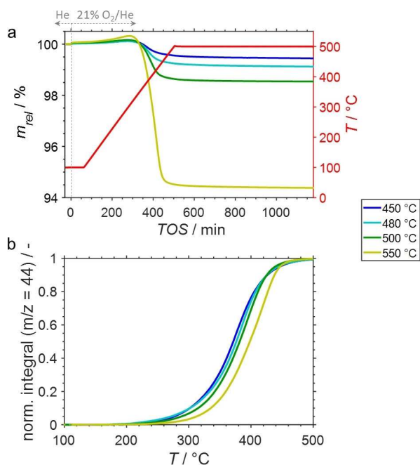
Figure 2. (a) Sample weight relative to the weight prior to exposure to 21 % O 2 /He at 100 °C and (b) normalised cumulative formation of CO 2 during temperature programmed oxidation (1 °C min −1 ) of spent SCALMS with an atomic Ga/Rh ratio of 125 as monitored via high-resolution thermogravimetry coupled with mass spectrometry. The catalysts were previously applied in propane dehydrogenation at 450, 480, 500, and 550 °C. Conditions of the experiment: He flow 100 mL min −1 for TOS < 0; He flow 79 mL min −1 and O 2 flow 21 mL min −1 for TOS > 0; GHSV 30000 mL g −1 h −1 .
