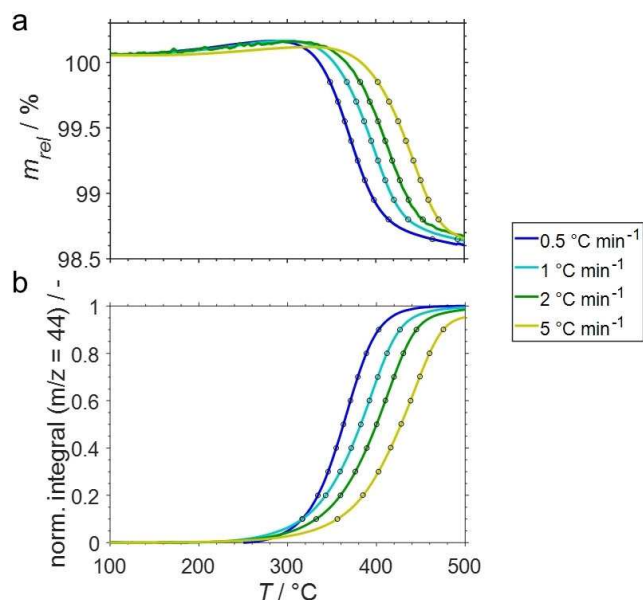
Figure 5. (a) Sample weight relative to the weight prior to exposure to 21 % O 2 /He at 100 °C (solid) and (b) normalised cumulative formation of CO 2 (solid) together with selected data points for isoconversional analysis (10–90 %, open circles) during temperature programmed oxidation of spent SCALMS with an atomic Ga/Rh ratio of 125 as monitored via high-resolution thermogravimetry coupled with mass spectrometry. The catalyst was previously applied in propane dehydrogenation at 500 °C. Conditions of the experiment: He flow 100 mL N min -1 for TOS < 0; He flow 79 mL N min -1 and O 2 flow 21 mL N min -1 for TOS > 0; GHSV 30000 mL N g -1 h -1 .
